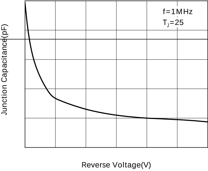
Fig.2:Capacitance Characteristics
